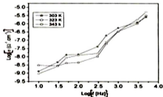
Fig.3 Variation of Log \sigma with frequency at different temperature for PMMA 75-PS25 film
